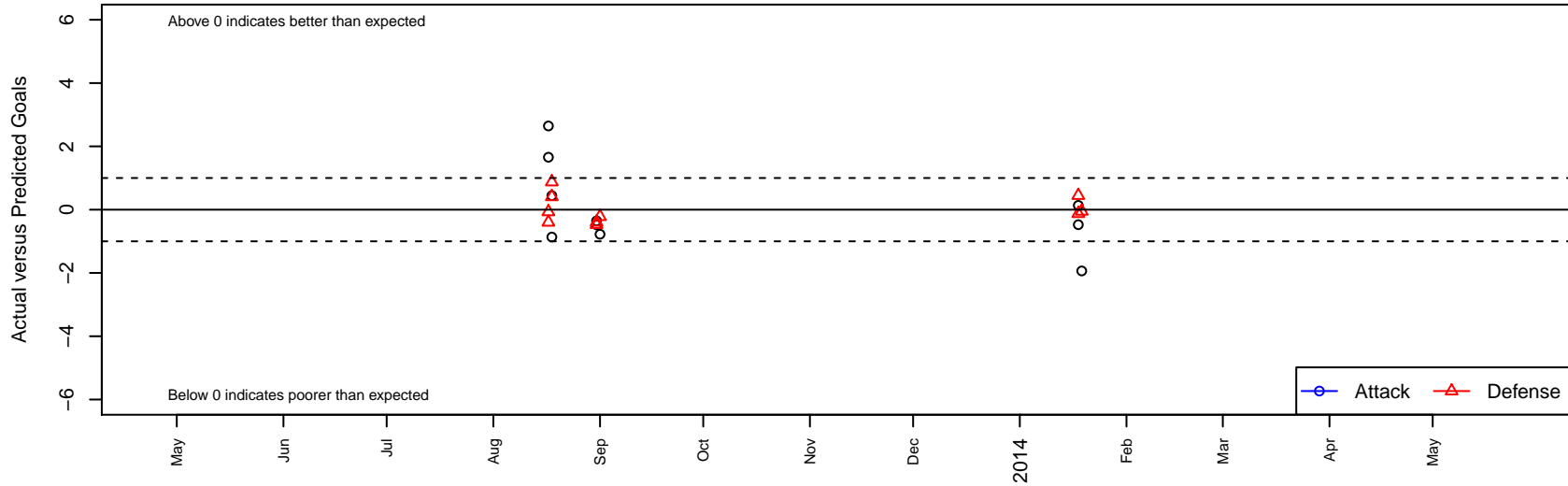
San Diego Crusaders SC Red G00 Dots are actual minus expected GF (blue circles) and GA (red triangles). Blue line is smoothed change in attack strength. Red is smoothed change in defense strength.
